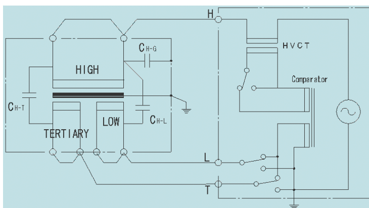
Power Transformer
