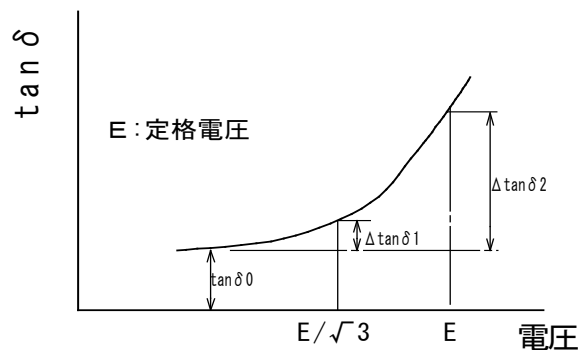
Tan Delta Test (tan δ)
