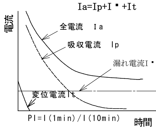
DC Absorption Test
